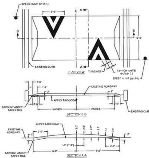
SPEED HUMP DETAIL
