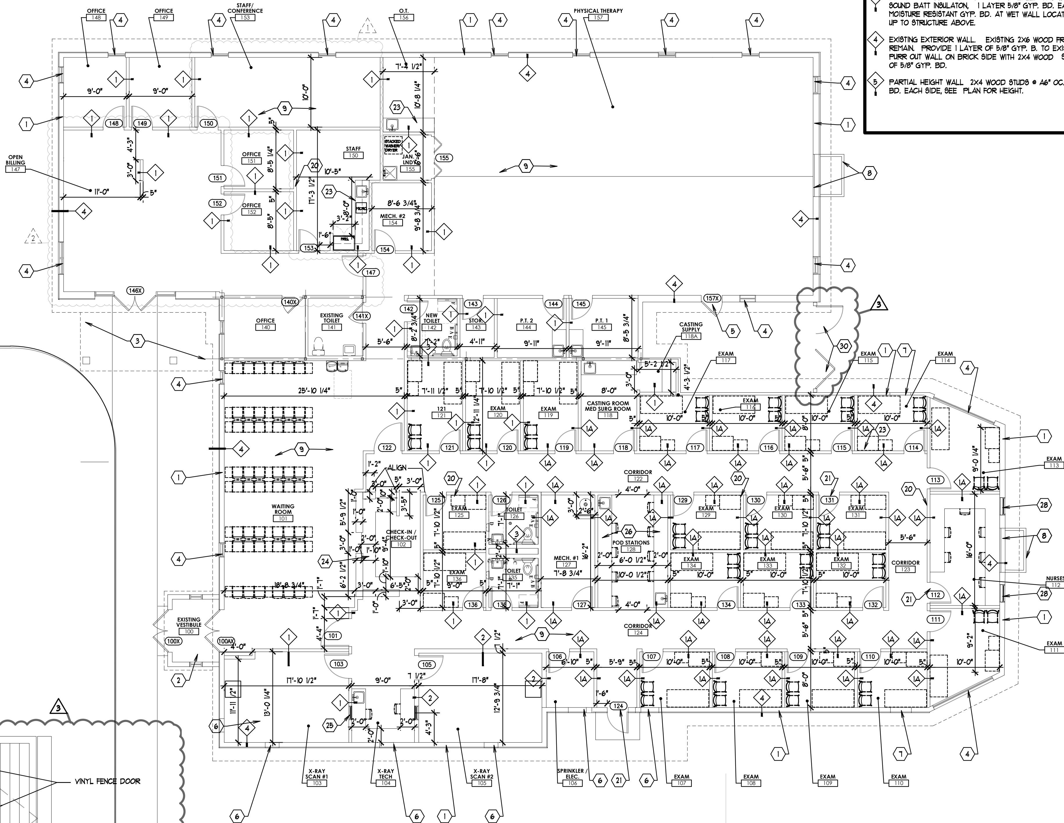
PROPOSED FLOOR PLAN 1/8" = 1'-0" A1.0
